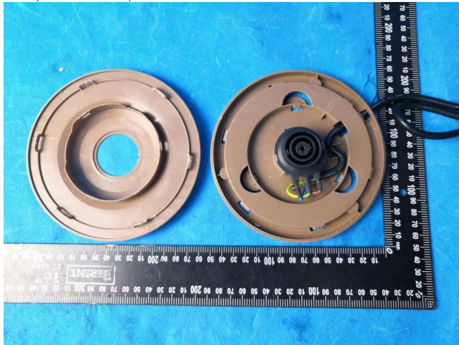
Internal view of stand, TPSK7318-15, TPSK7318-18
