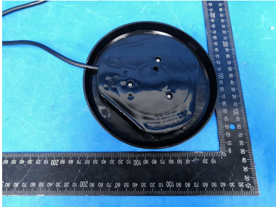
Overall view, TPSK8518-15, TPSK8518-18, stand bottom
