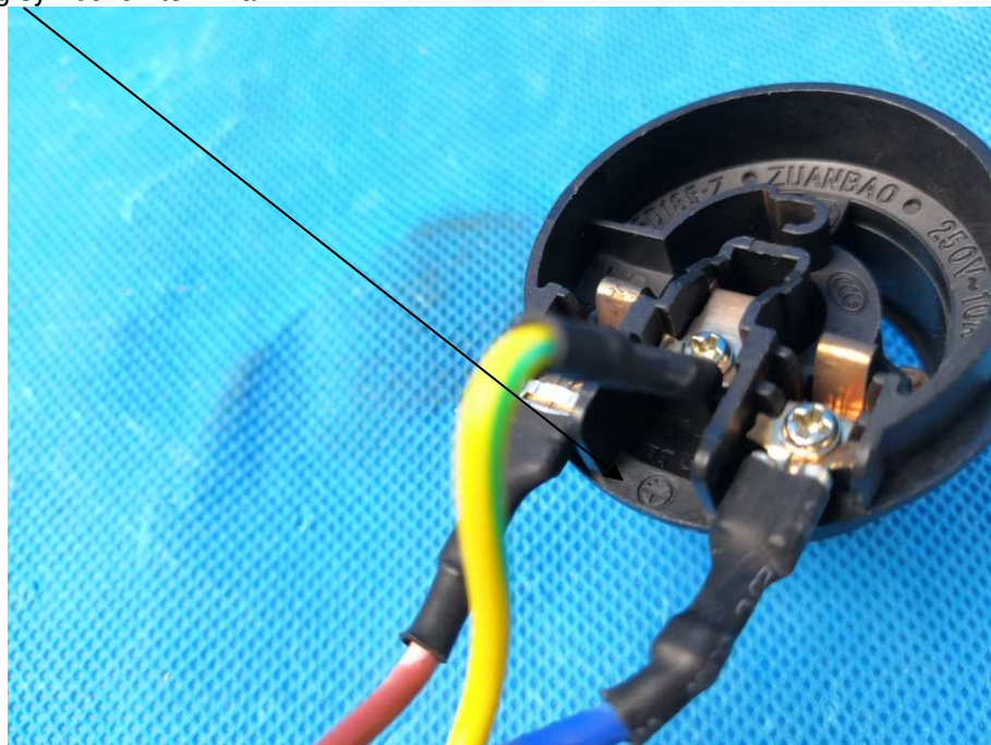
View of earthing symbol on terminal
