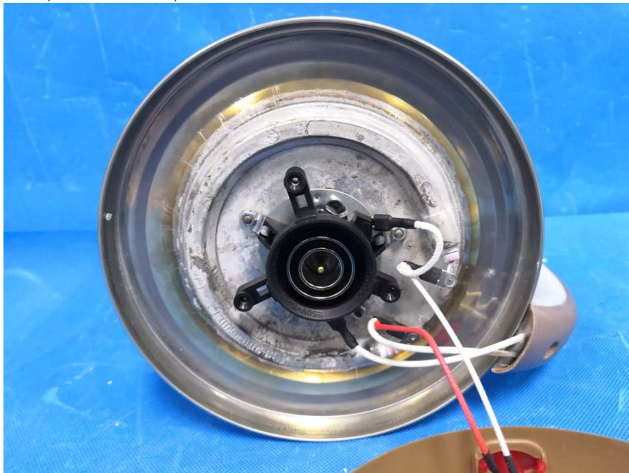
Internal view of kettle, TPSK7625-15, TPSK7625-18
