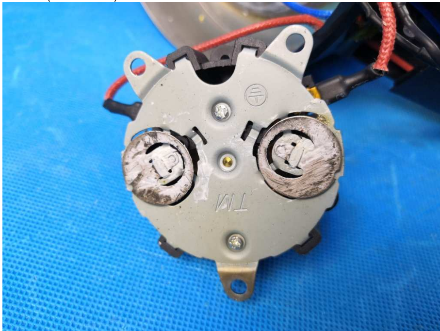
View of thermal control (TIANMING)
