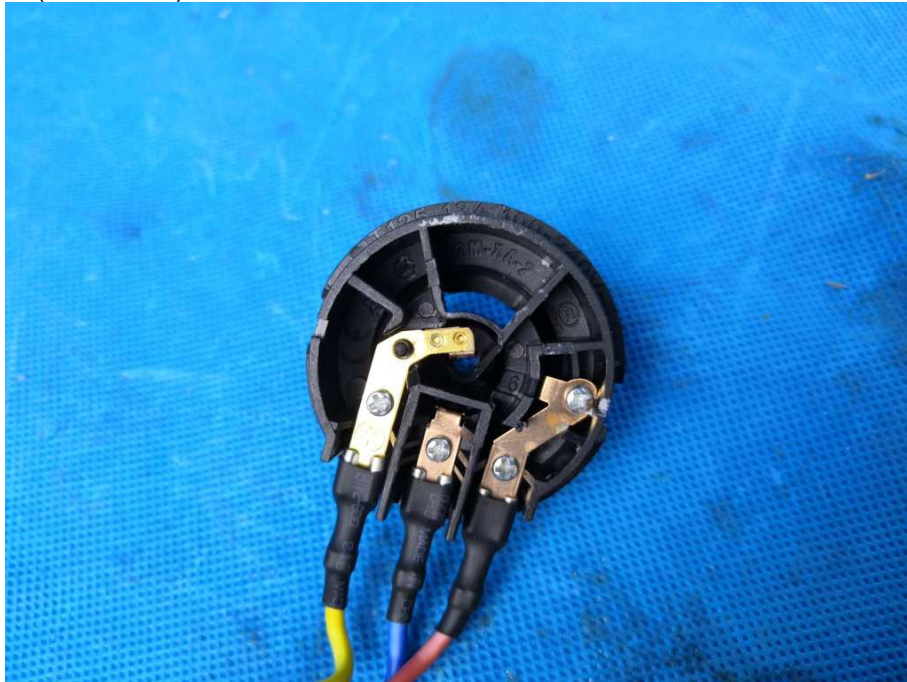
View of connector (TIANMING)
