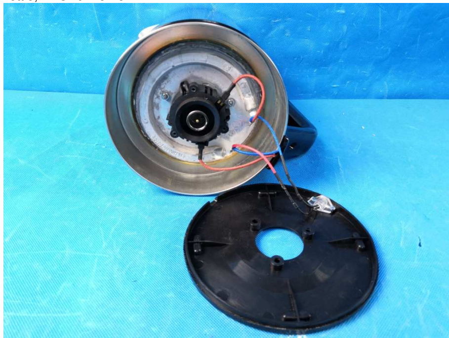
Internal view of kettle, TPCK0118-18
