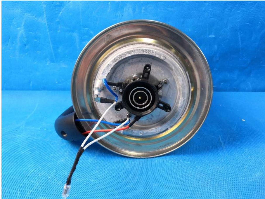
Internal view of kettle, TPSK0318-15, TPSK0318-18
