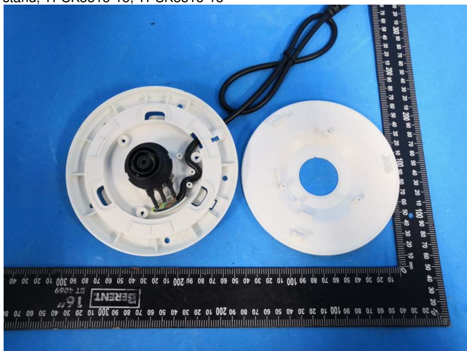
Internal view of stand, TPSK8815-15, TPSK8815-18
