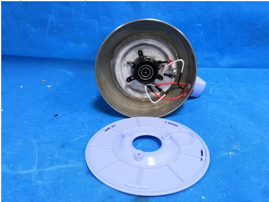
Internal view of kettle, TPSK5218SS-15, TPSK5218SS-18
